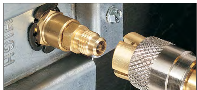
CM-SNAP SnapMate® Connector
