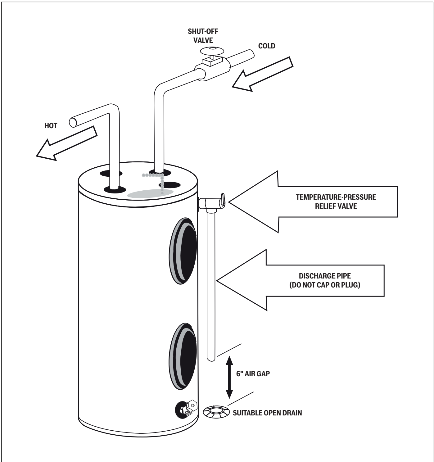
Figure 6 Installation Example
